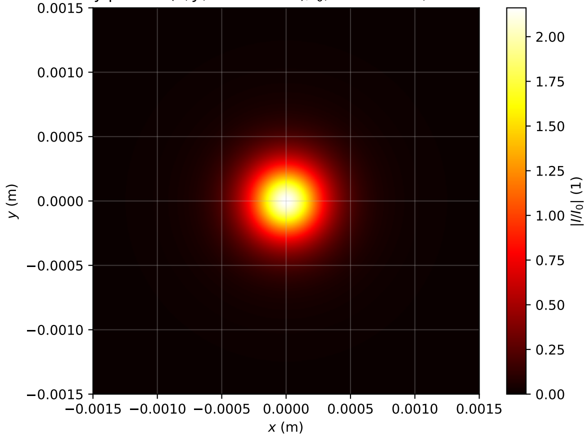
Intensity profile I(x, y, z = 2.070m)/I_0 , P_{in}=1.0P_{cr} , artificial time
